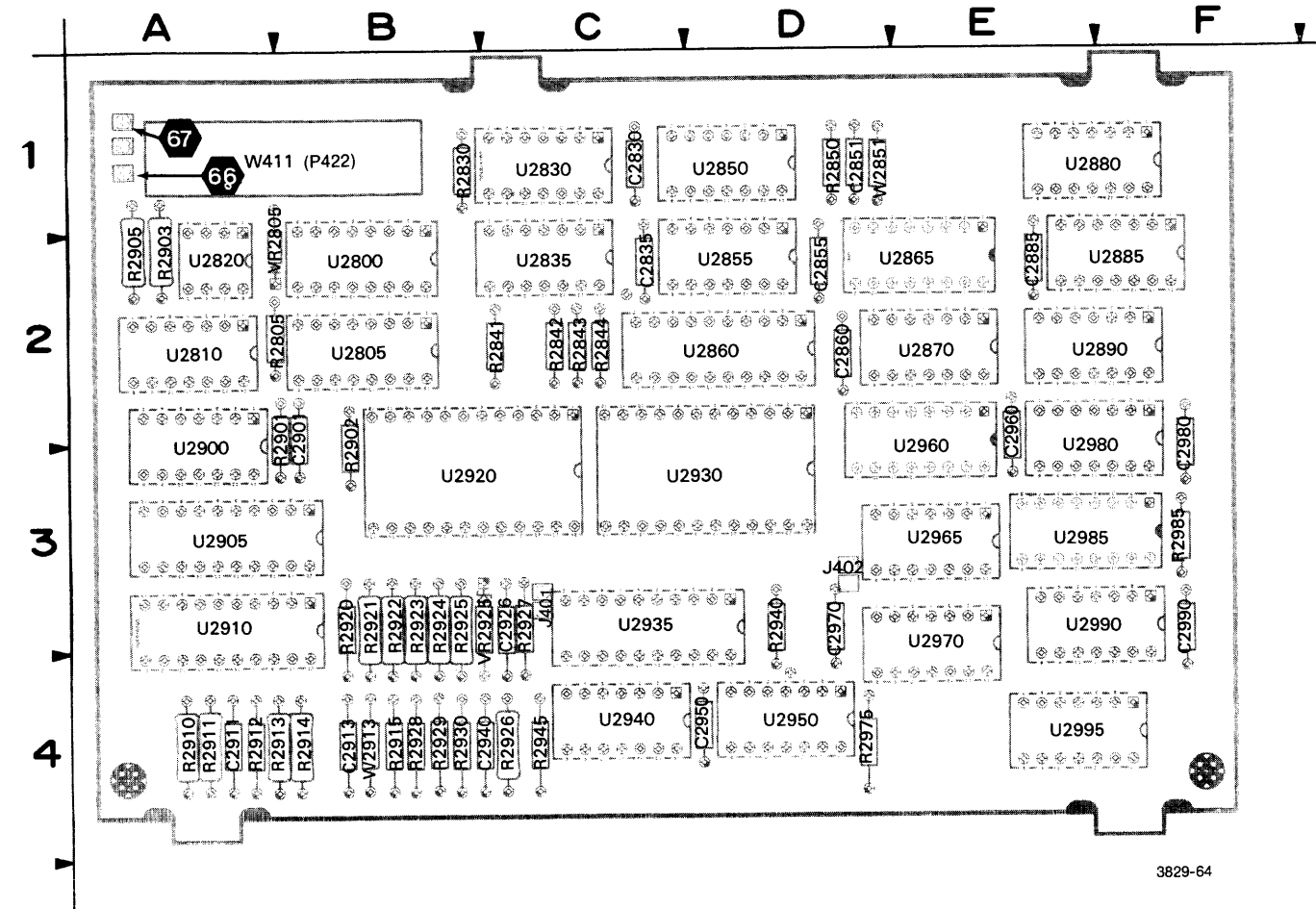
Figure 9-10. A4—Readout board.
