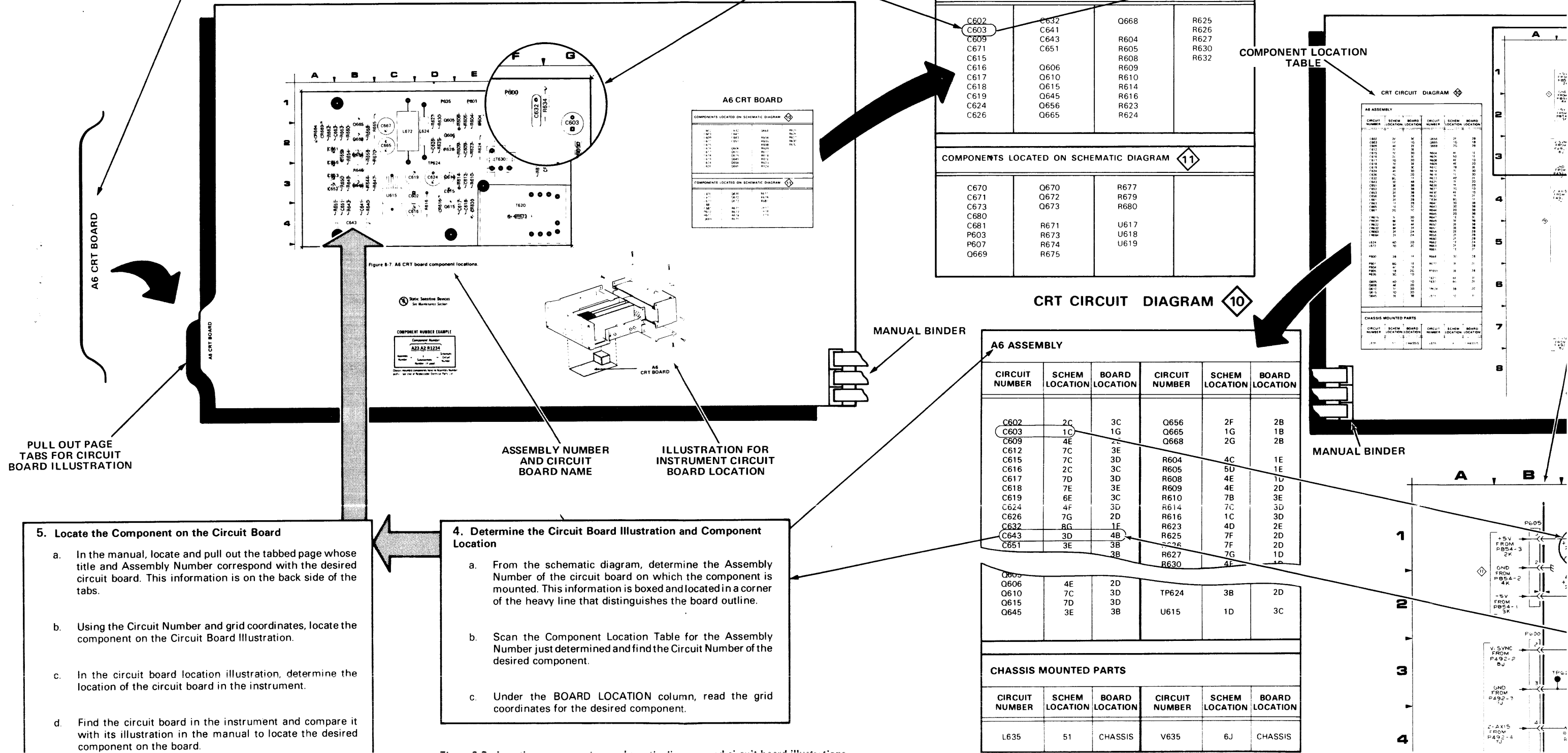
Figure 9-3. Locating components on schematic diagrams and circuit board illustrations.
